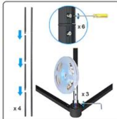
Step 2: Assembly 4 aluminum tubes into lamp base.
