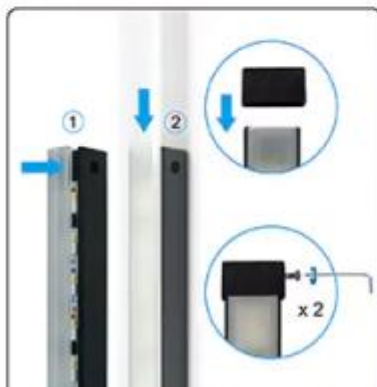
Step 4: Assembly lens cover by press into or (insert to) aluminum tubes and assembly lamp cap.
